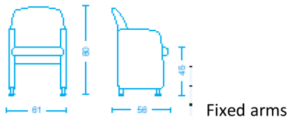
Fixed arms
